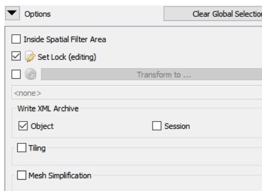
Figure 5.2 Download Options
