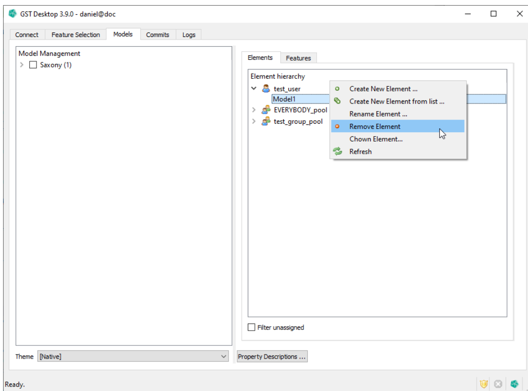
Figure 9.6 Remove Modell
