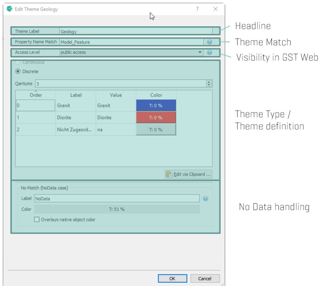
Figure 12.1 Theme Editor
