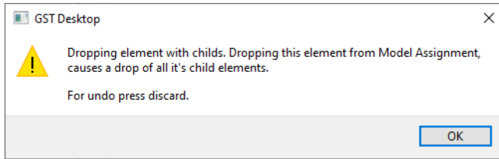
Figure 9.16 Warning dialog
