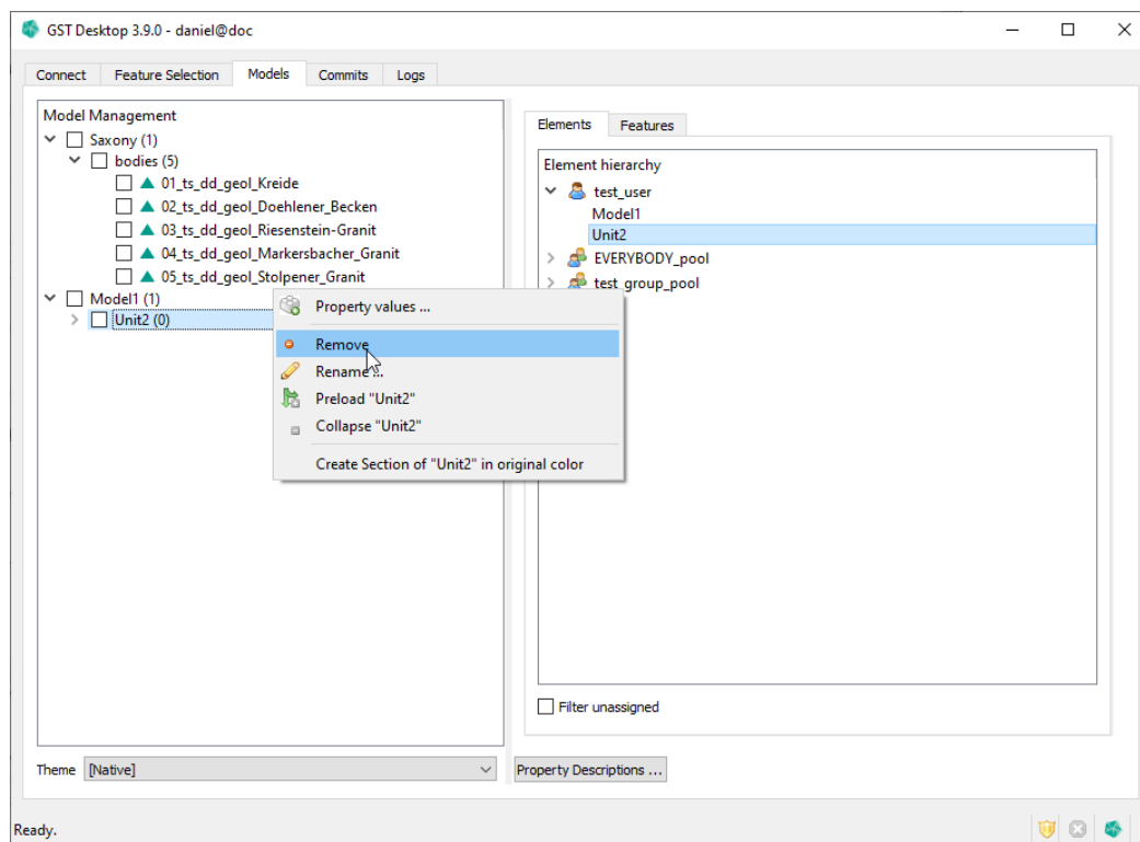
Figure 9.15 Unassign element
