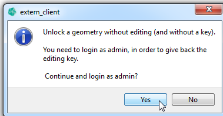
Figure 6.9 Confirmation dialog
