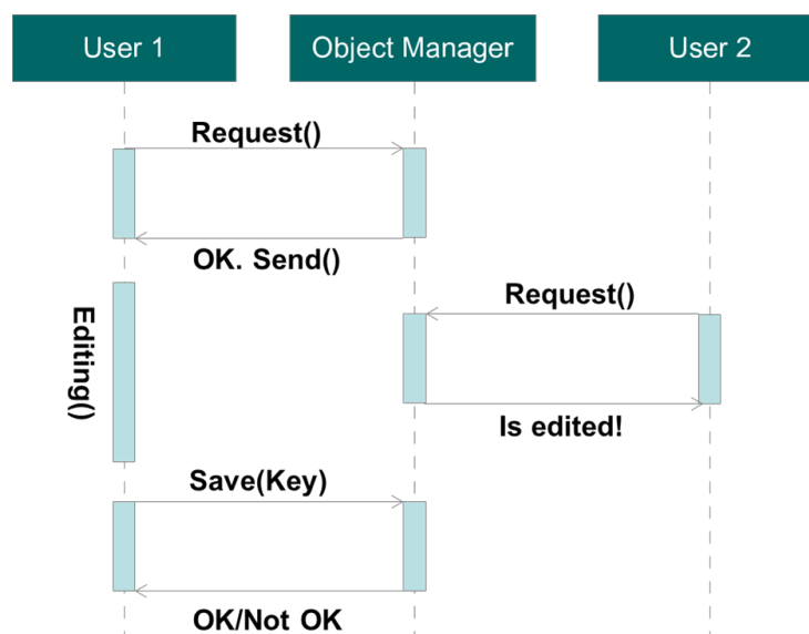
Figure 6.5 Changing data requires a lock key
