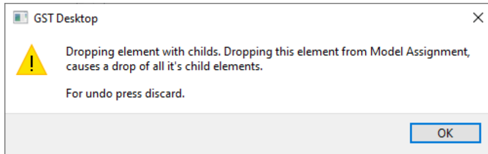
Figure 10.16 Warning dialog
