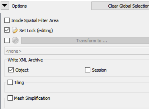
Figure 6.2 Download Options
