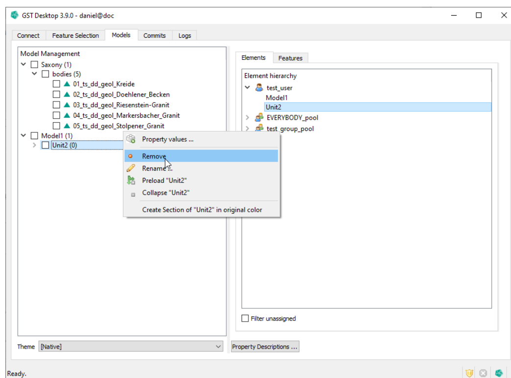
Figure 10.15 Unassign element
